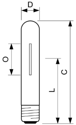
Agro/GreenPower, 250W/400W/600W
